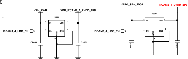
RCAM3_4_AVDD
